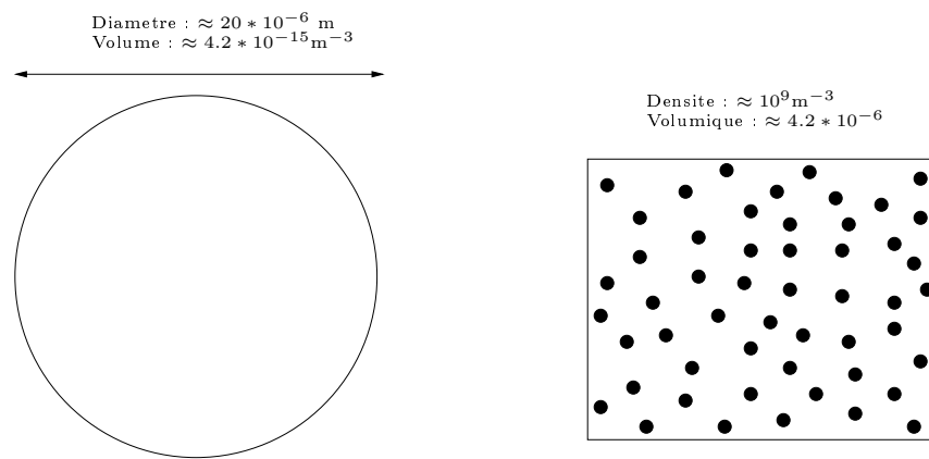
FIG. 1 – Cloud characteristics
