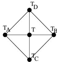
Figure 3: Simple triangulation for building a monotone update operator.
