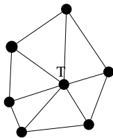
Figure 4: Acute triangulation around center grid point.
