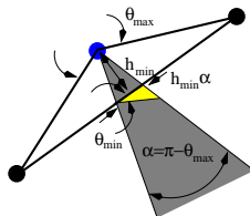
Figure 7: The smallest possible area of one triangle covered by the longest possible extended section bounds the number of unfolded triangles. The triangle with a_{min} is the bright shaded one.
