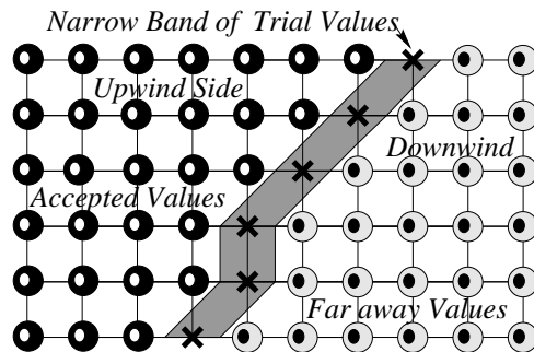
Figure 1: Upwind construction of accepted values.
