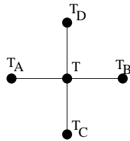
Figure 2: Construction of upwind solution on orthogonal mesh.
