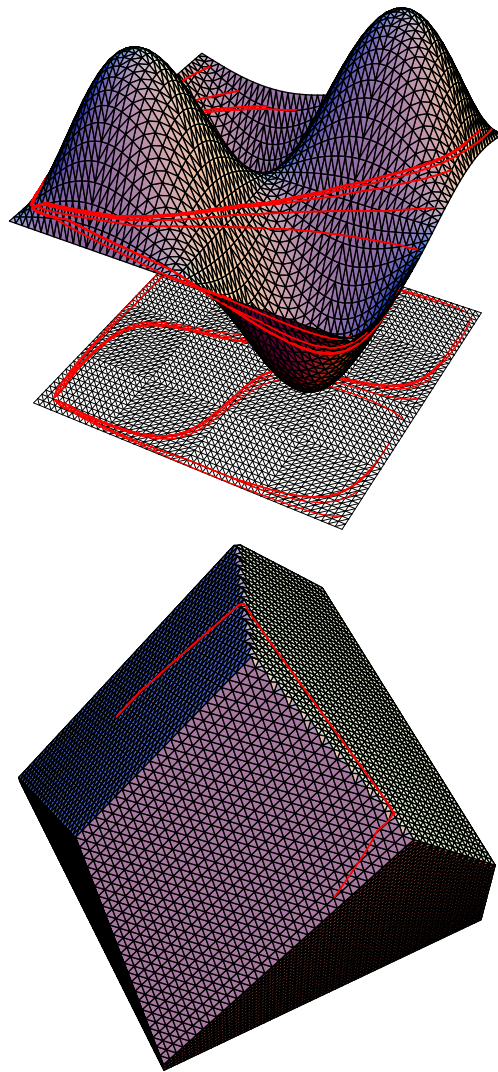
Figure 8: Computing minimal weighted geodesics on triangulated surfaces.
