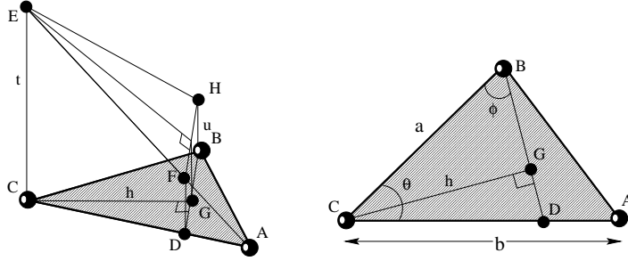
Figure 5: Given the triangle ABC , such that u = T(B) - T(A) , find T(C) = T(A) + t such that (t - u)/h = F . Left: A perspective view of the triangle stencil supporting the T() values that form a tilted plane with a gradient magnitude equal to F . Right: The trigonometry on the plane defined by the triangle stencil.
