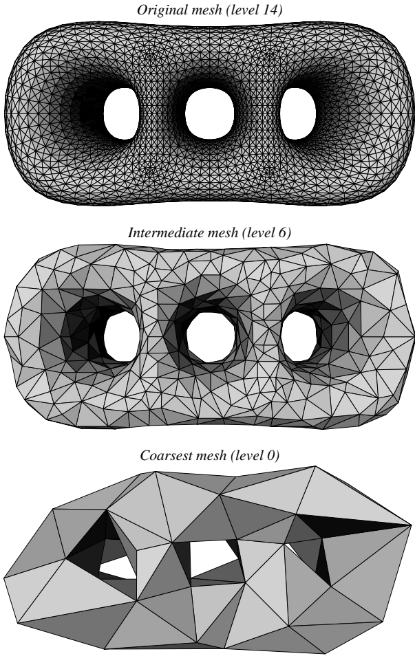
Figure 4: Example of a modified DK mesh hierarchy. At the top the finest (original) mesh \varphi(|K^L|) followed by an intermediate mesh, and the coarsest (base) mesh \varphi(|K^0|) at the bottom (original dataset courtesy University of Washington).
