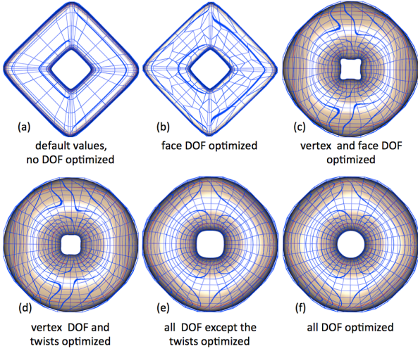
Figure 8: Optimization of different subsets of degrees of freedom. All remaining DOF are set with default values. The optimized subsets of DOF are respectively from left to right: (a) no DOF optimized, (b) face DOF, (c) vertex and face DOF, (d) vertex DOF and twists, (e) all DOF without twists, (f) all DOF. The input mesh is the torus mesh of Figure 10, second row. The Bézier control net and isophotes are drawn in blue.
