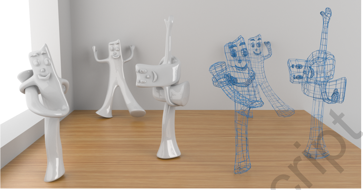
Figure 2: Irregular quad meshes interpolated by a G^1 -continuous surface composed of biquartic Bézier patches. Each object is composed of nine independent genus 0 meshes representing the body and the face elements separately.
